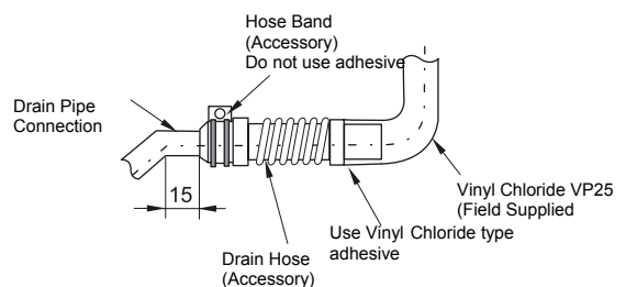
Hose Band (Accessory)
